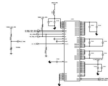
Direct Charging
