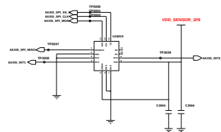
6 AXIS SENSOR (GYRO,ACCEL)
